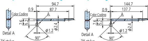
12AAC740 (2µm)* ( ) : Tip radius 12AAB413 (5µm)** *Tip angle: 60° 12AAB425 (10µm)** **Tip angle: 90° 12AAC741 (2µm)* ( ) : Tip radius 12AAB414 (5µm)** *Tip angle: 60° 12AAB426 (10µm)** **Tip angle: 90°
