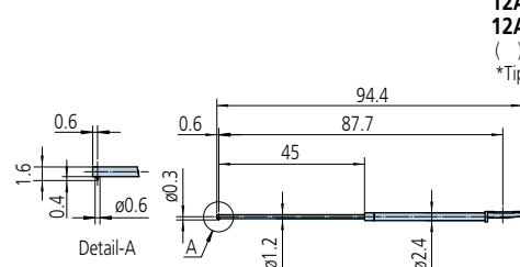
12AAC740 (2µm)* ( ) : Tip radius 12AAB413 (5µm)** *Tip angle: 60° 12AAB425 (10µm)** **Tip angle: 90° 12AAC741 (2µm)* ( ) : Tip radius 12AAB414 (5µm)** *Tip angle: 60° 12AAB426 (10µm)** **Tip angle: 90°
