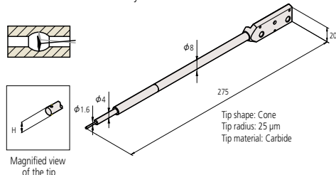
• Double small-hole arm stylus: 12AAM108/12AAT469
