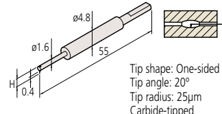
Small hole stylus SPH-41
