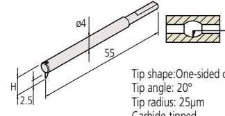
Small hole stylus SPH-43
