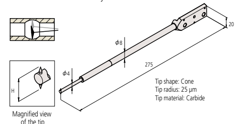
• Double small-hole arm stylus: 12AAM110
