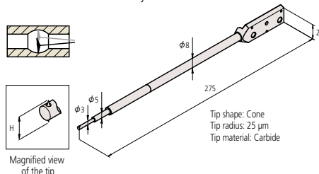
• Double small-hole arm stylus: 12AAM109/12AAT470
