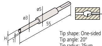
Small hole stylus SPH-42
