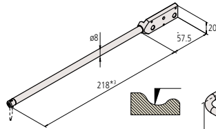
• Straight arm AB-31
